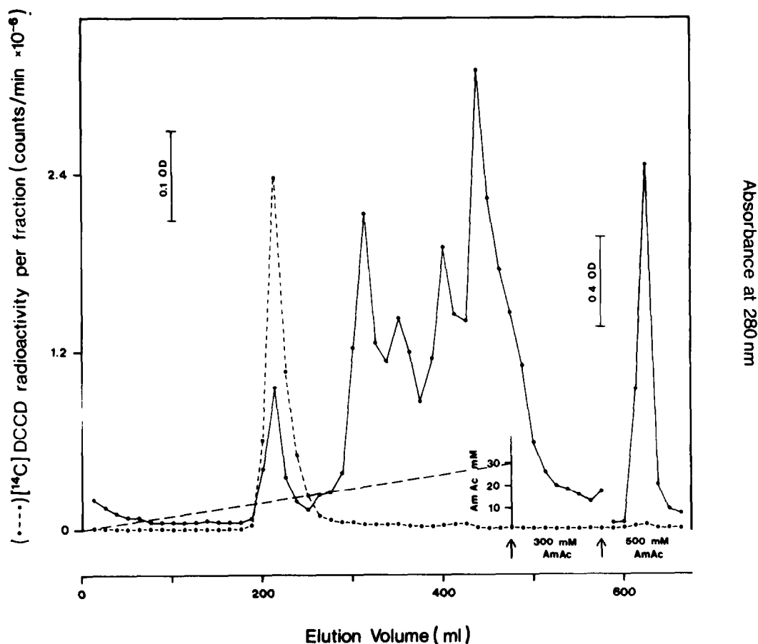
Fig.2. CM-cellulose chromatography of the crude proteolipid fraction isolated from [ 14 C]DCCD-labelled submitochondrial particles of beef heart. The crude proteolipid (46 mg) dissolved in 46 ml chloroform/methanol (2/1) was applied to a CM-cellulose column of 40 ml bed volume. The column was then washed successively with 50 ml chloroform/methanol (2/1), 100 ml chloroform/methanol (1/1) and 50 ml chloroform/methanol/water (5/5/1). The proteins were then eluted with, first 500 ml of a linear ammonium acetate gradient (0–30 mM) at a flow rate of 50 ml/h, secondly 100 ml 300 mM ammonium acetate and, thirdly 100 ml 500 mM ammonium acetate, all in the presence of chloroform/methanol/water (5/5/1). A_{280} (●—●) and [ 14 C]DCCD radioactivity (●—●) were determined in 12.5 ml fractions.
